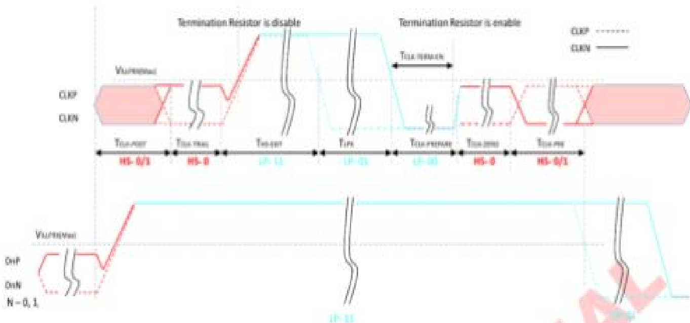
Clock Lane –High speed mode to / from Low Power Mode Timing
