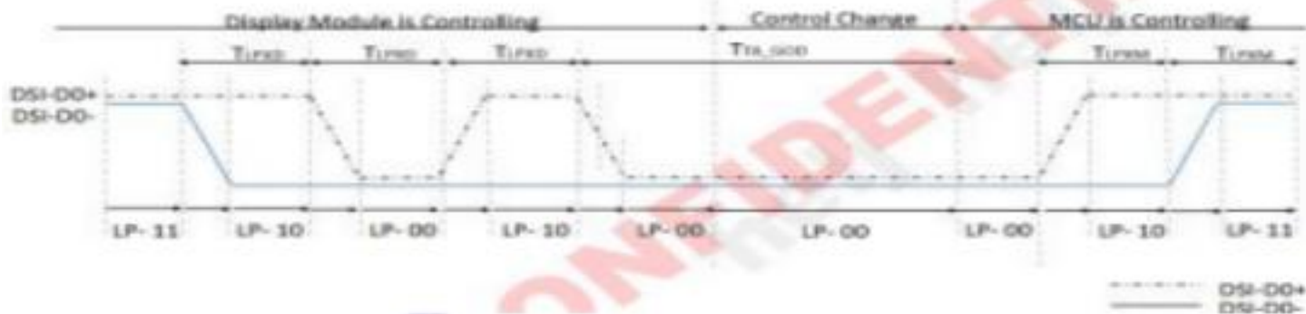
Low Speed Mode - Bus Turn Around Timing
