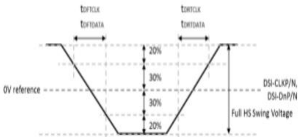
Figure 6-2 Rising and Falling Timings
