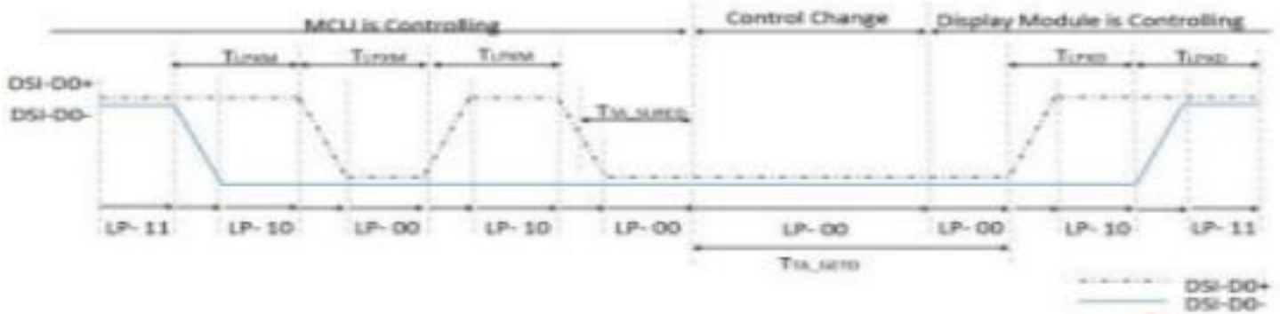
Bus Turnaround (BTA) from MCU to display module Timing
