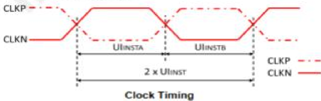
High Speed Mode - Clock Timing
