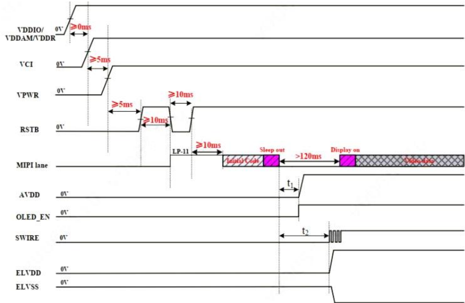
Fig 1 Power on sequence
