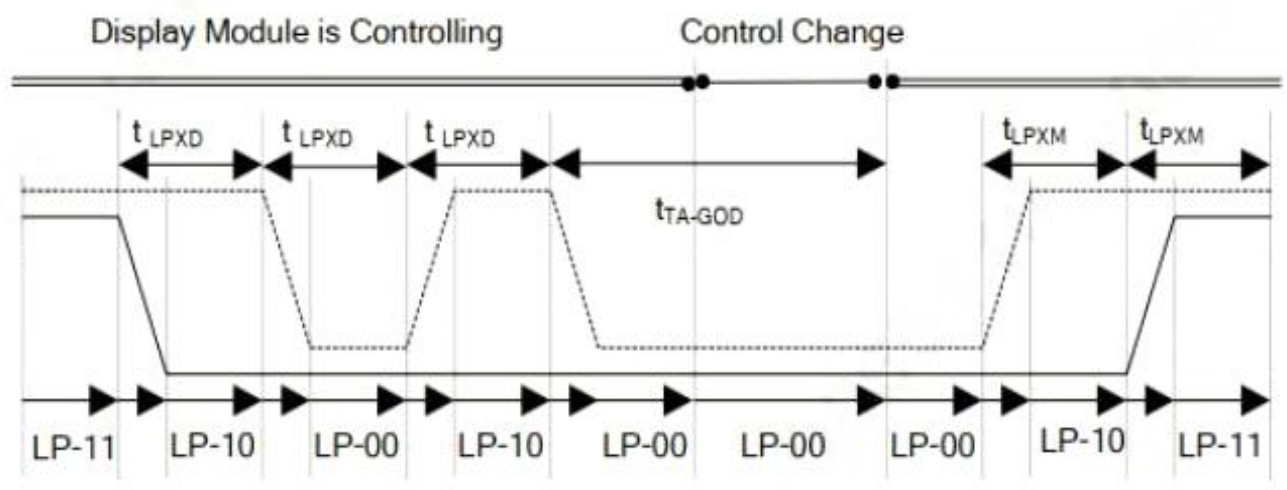
Bus Turnaround (BAT) from display module to MPU Timing
