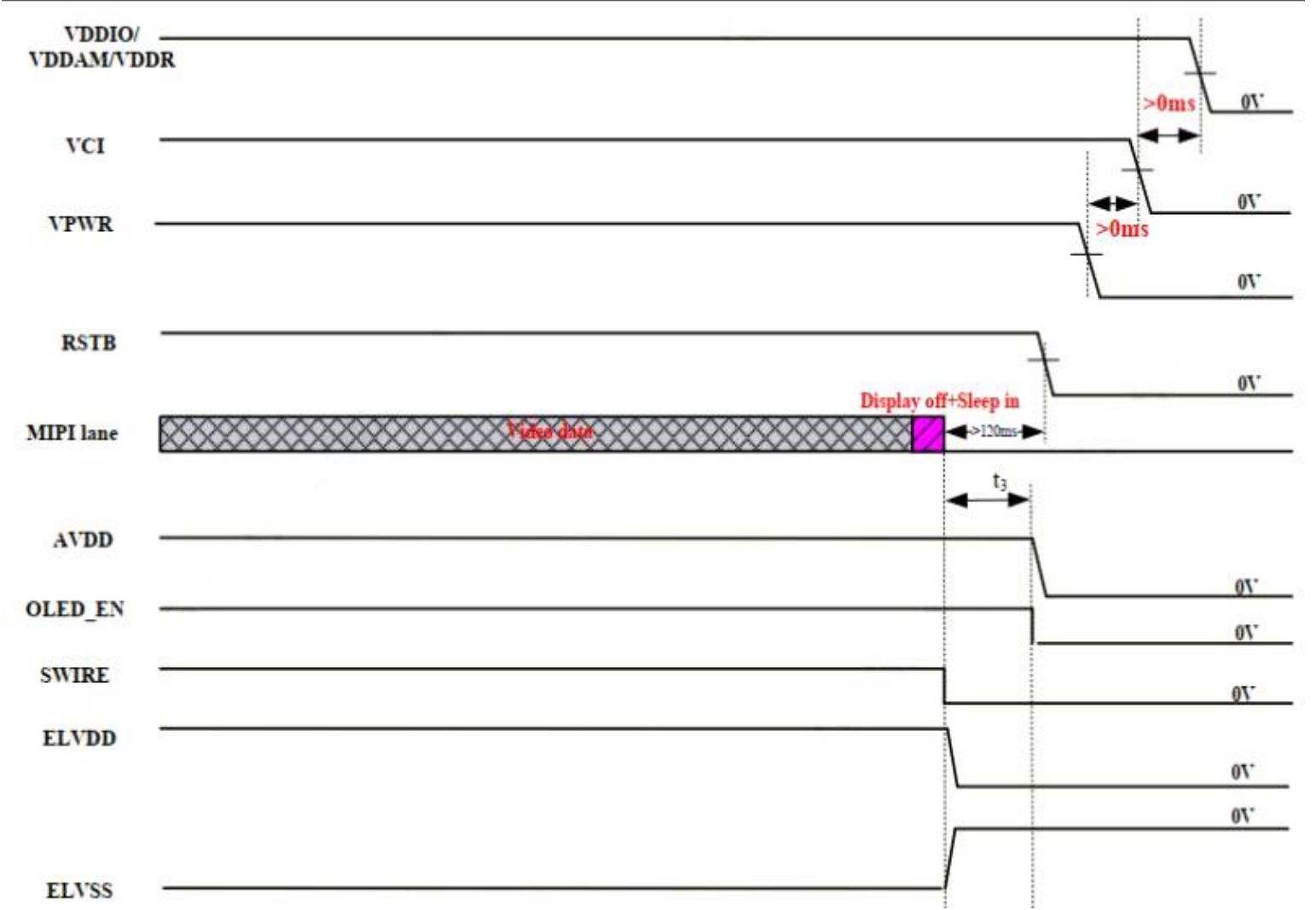
Fig 2 Power off sequence
