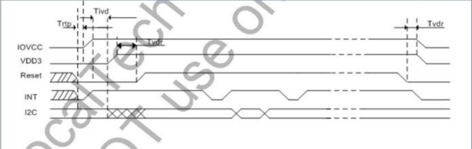
Figure 3-6 Power on-off Sequence
