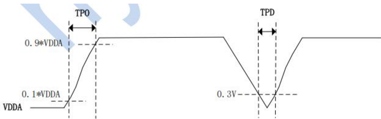
Power-up sequence
