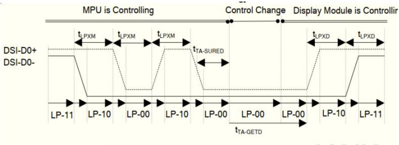
Bus Turnaround (BAT) from MPU to display module Timing
