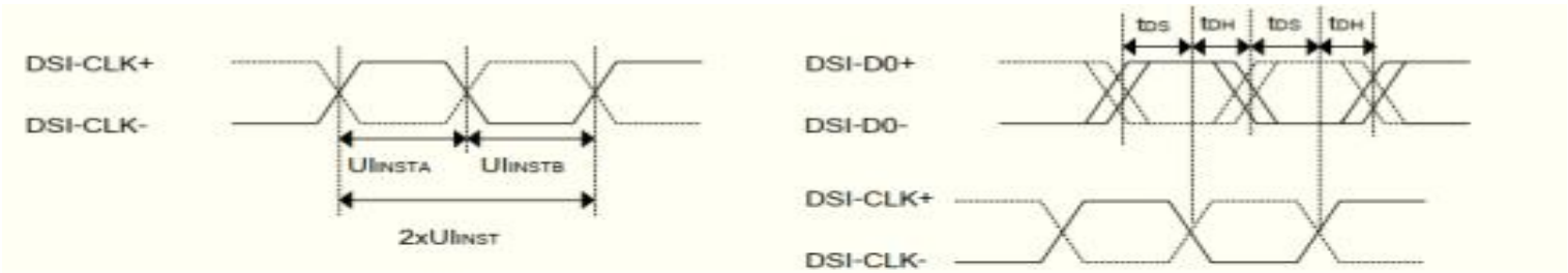
DSI clock channel timing
