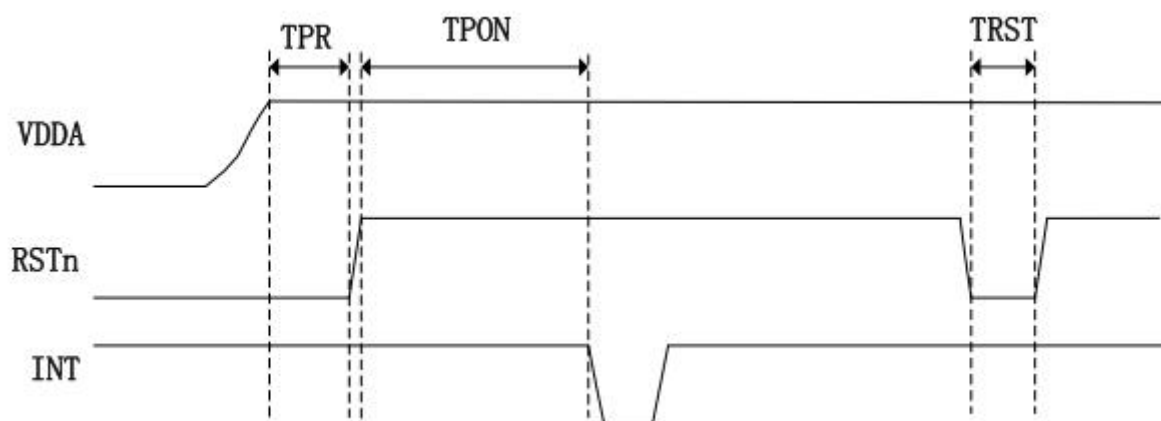
Reset timing sequence
